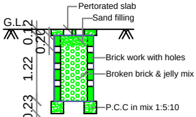
PERCOLATION PIT FOR 30 Sq. m. (Scale:- 1:50)
