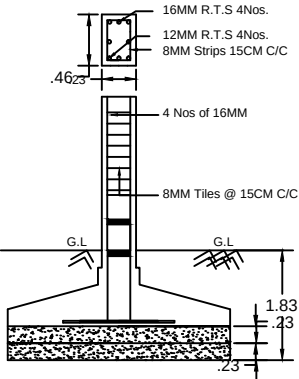
RCC COLUMN DETAILS
