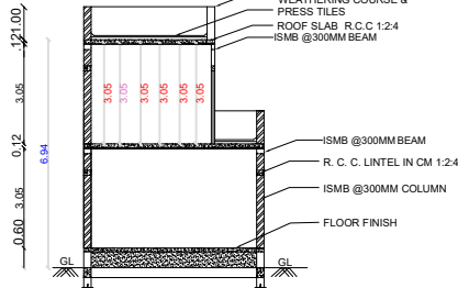
SECTION ON AB & (HALF ELEVATION)
