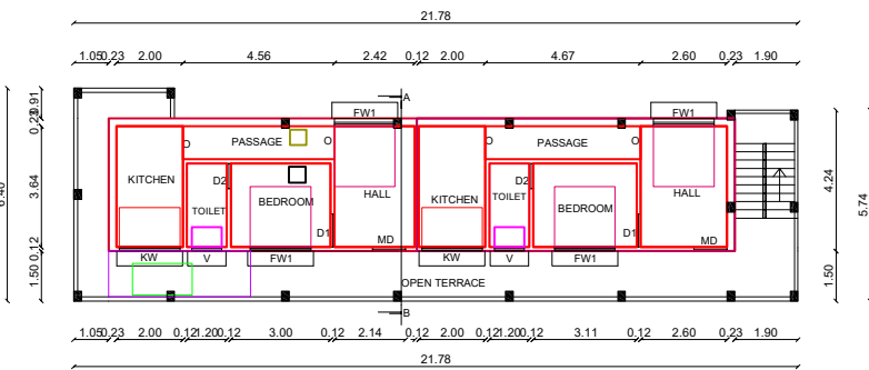
FIRST FLOOR PLAN PROPOSED
