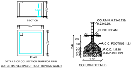
DETAILS OF COLLECTION SUMP FOR RAIN WATER HARVESTING OF ROOF TOP RAIN WATER RWH_CAPACITY_L=5000LTRS
