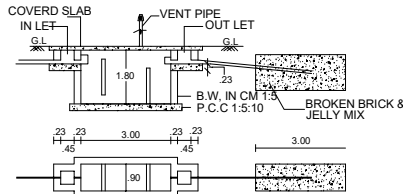
PLAN & SECTION OF SEPTIC TANK & TRENCH
