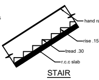
STAIR
