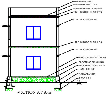
SECTION AT A-B
