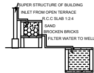
RAINWATER HARVESTING
