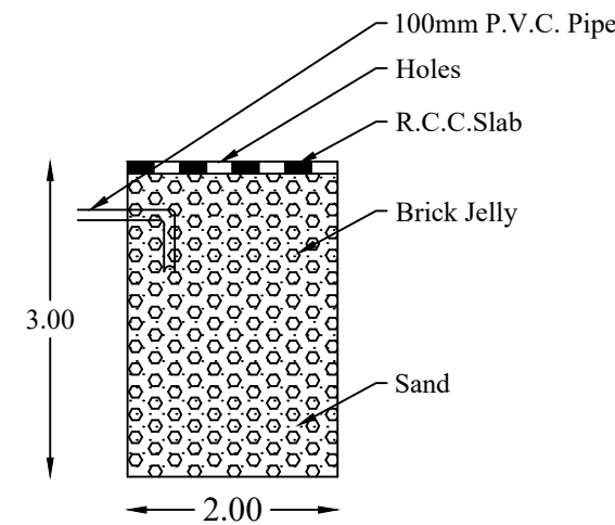
SECTION OF RAIN WATER COLLECTING TANK
