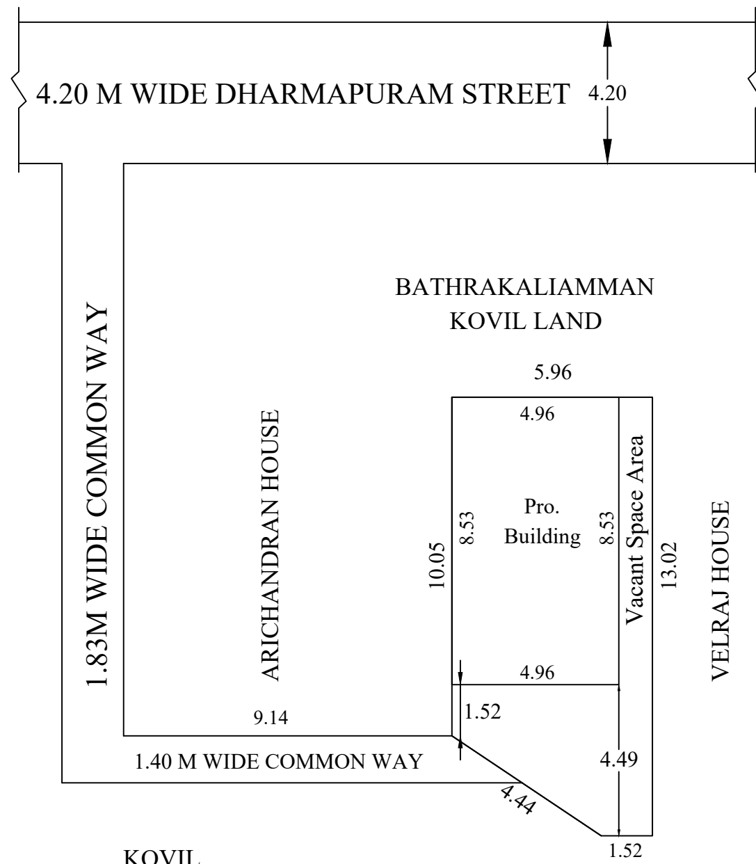
SITE PLAN
