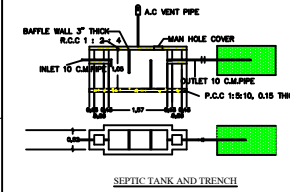
Septic Tank
