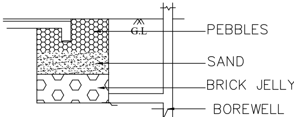
RAINWATER FILTRATION
