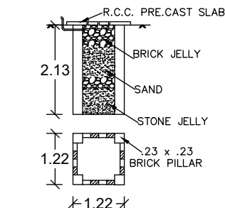
PLAN & SECTION OF RAIN WATER COLLECTION WELL
