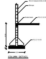
COLUMN DETAIL
