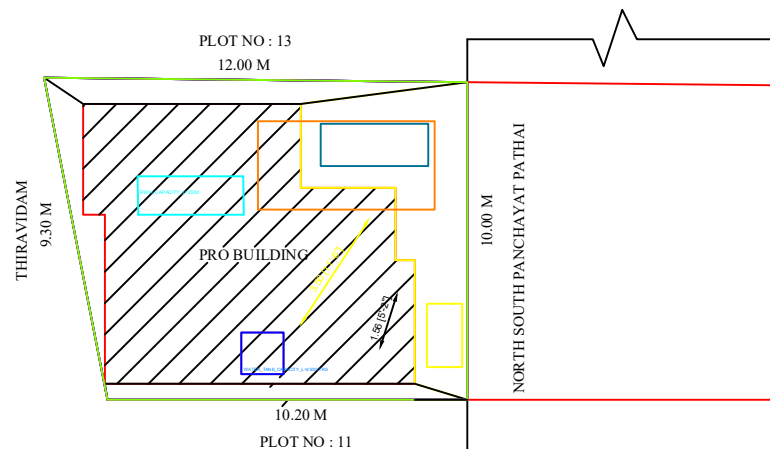
SITE PLAN
