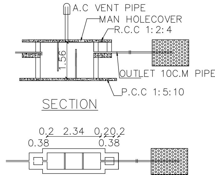
PLAN OF SEPTIC TANK & TRENCH
