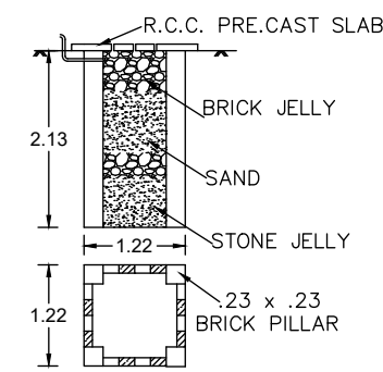
PLAN & SECTION OF RAIN WATER COLLECTION WELL
