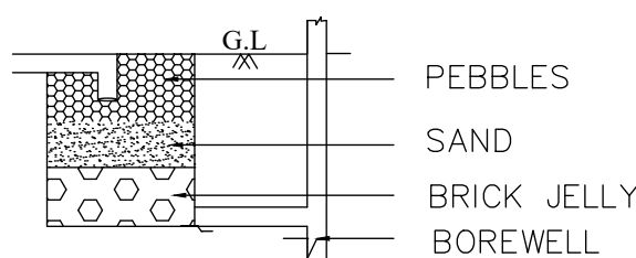
RAINWATER FILTRATION
