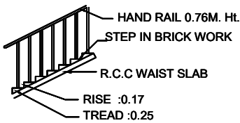
STAIR CASE DETAIL
