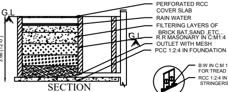
RAIN WATER HARVESTING OF RECHARGE TRENCH METHOD
