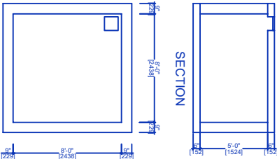
DETAILS OF COLLECTION SUMP FOR RAIN
