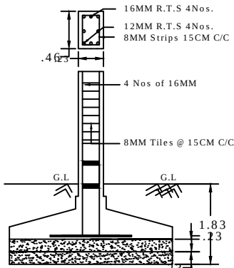
RCC COLUMN DETAILS
