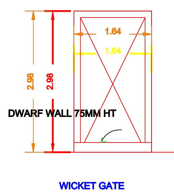
WICKET GATE
