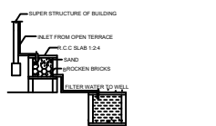
DETAILS OF FILTER BED & WELL NTS
