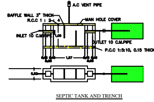
Septic Tank
