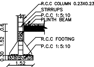
COLOUMN DETAILS
