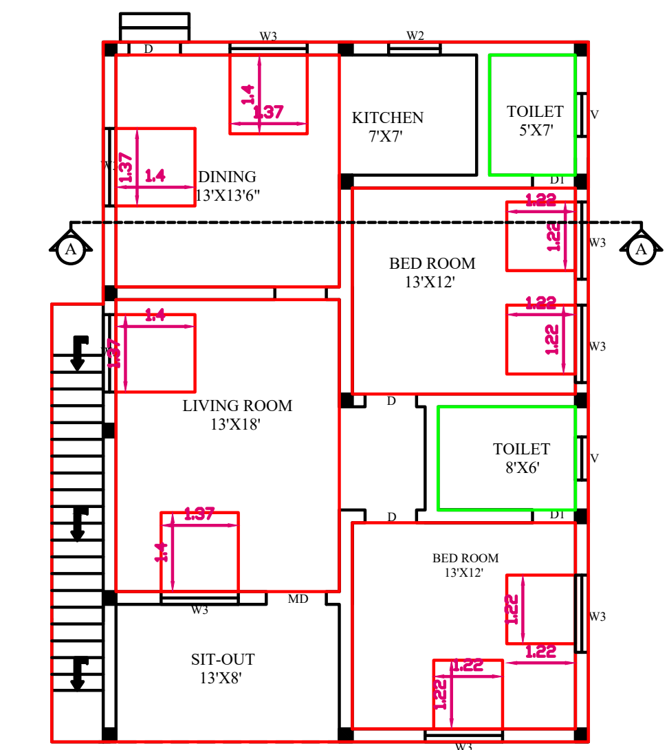
PRO.GOUND FLOOR PLAN
