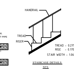
STAIRCASE DETAILS
