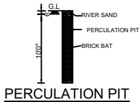
PERCOLATION PIT
