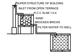
RAINWATER HARVESTING
