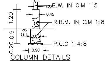
COLUMN DETAILS
