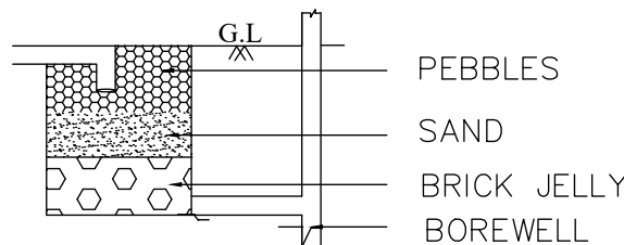
RAINWATER FILTRATION
