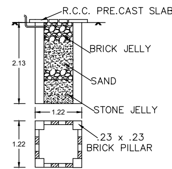
PLAN & SECTION OF RAIN WATER COLLECTION WELL
