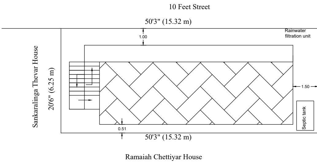
SITE PLAN
