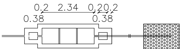
PLAN OF SEPTIC TANK & TRENCH
