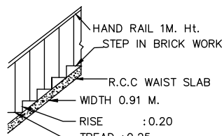
STAIR DETAIL
