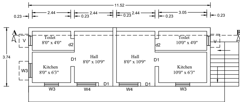
PROPOSED FIRST FLOOR PLAN
