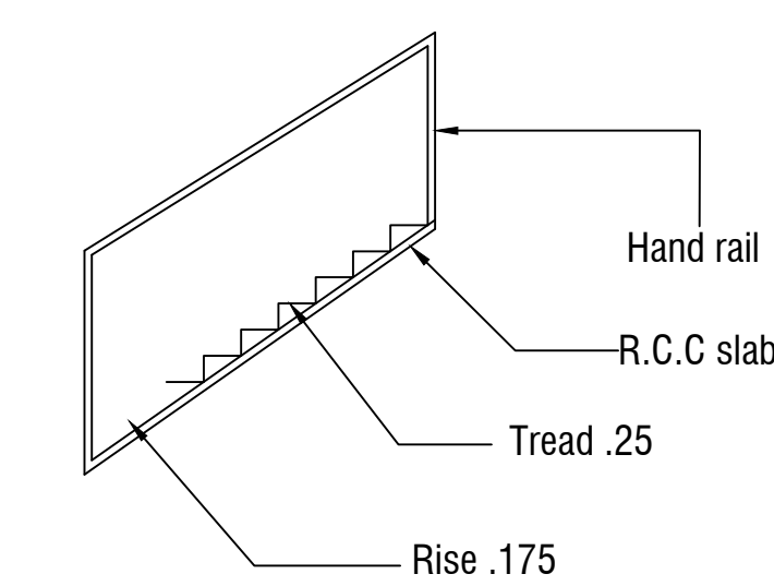
STAIR DETAIL
