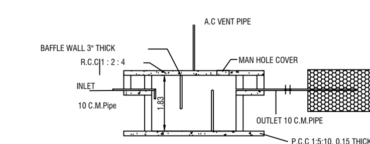
SEPTIC TANK AND TRENCH
