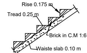
STAIR DETAILS
