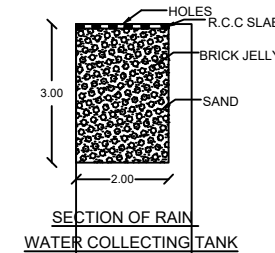
SECTION OF RAIN WATER COLLECTING TANK
