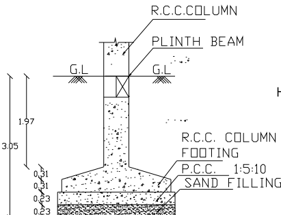
FOUNDATION DETAIL
