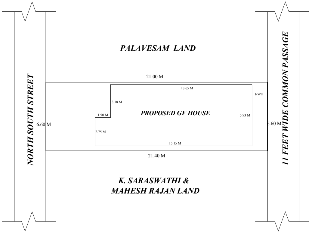
SITE PLAN
