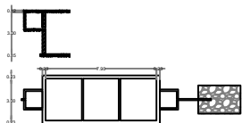
SEPTIC TANK AND TRENCH NTS
