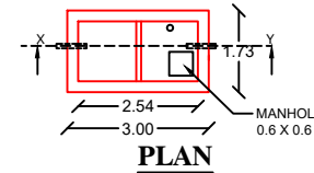
SEPTIC TANK
