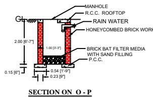
SECTION ON O - P
