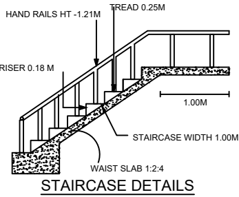
STAIRCASE DETAILS
