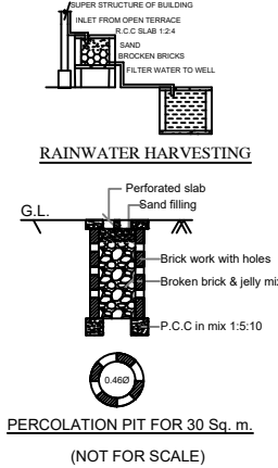
PERCOLATION PIT FOR 30 Sq. m. (NOT FOR SCALE)
