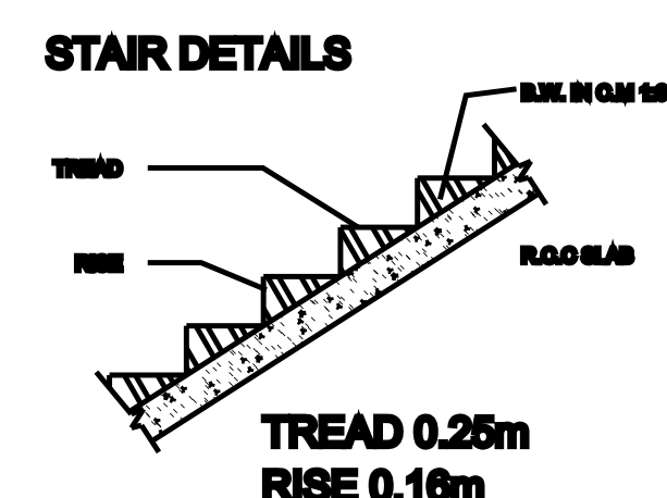
STAIR CASE
