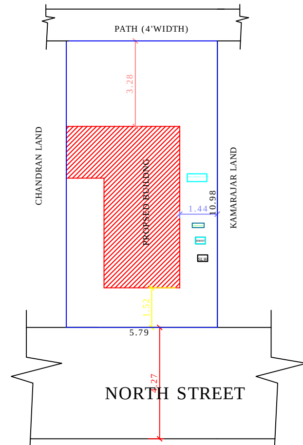
SITE PLAN
