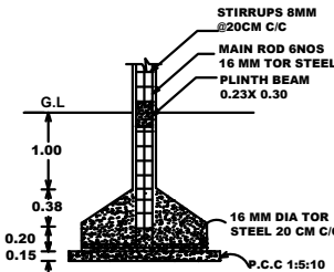
DETAILS OF COLUMN FOOTING
