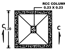
DETAILS OF COLUMN PLAN
