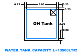
WATER_TANK_CAPACITY_L=13500LTRS
