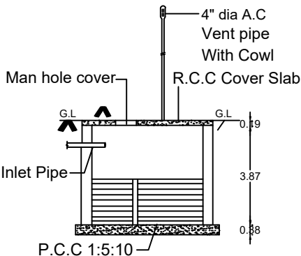
SECTION
