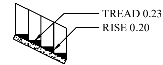
STAIR CASE DETAILS
