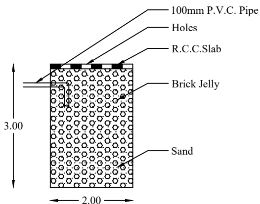
SECTION OF RAIN WATER COLLECTING TANK
