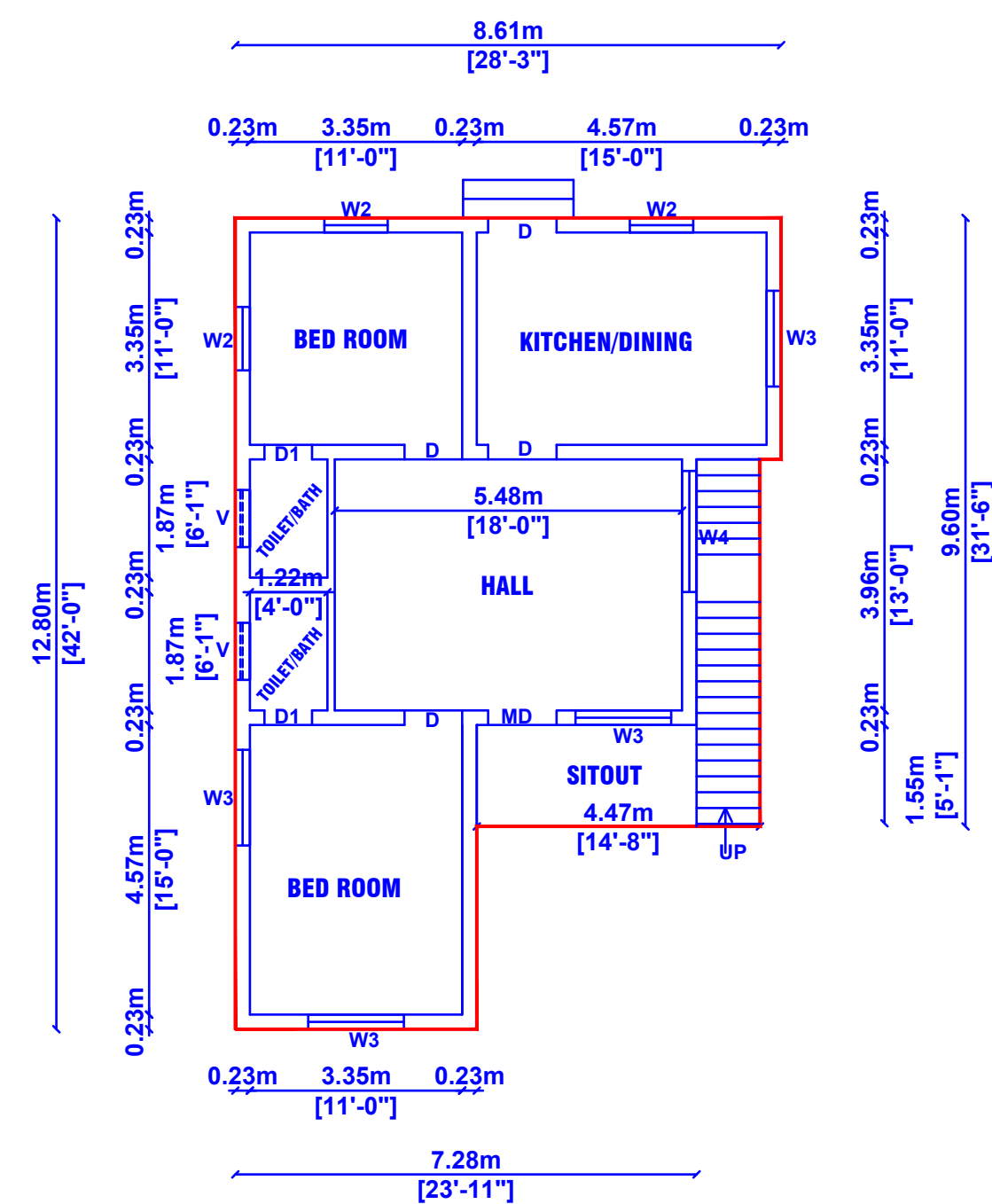
PLAN (Proposed)
