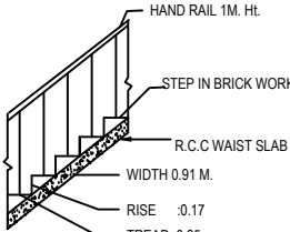
STAIR DETAIL
