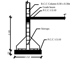
Column Detail
