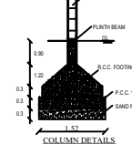
COLUMN DETAILS
