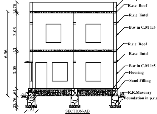
SECTION-AB
