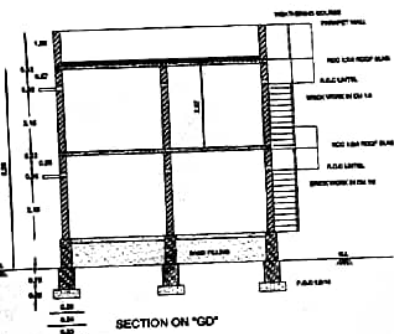
SECTION ON "GD"
