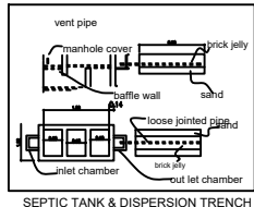
SEPTIC TANK & DISPERSION TRENCH
