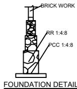
FOUNDATION DETAIL
