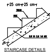
STAIRCASE DETAILS
