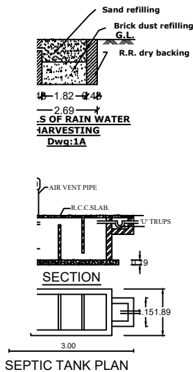
SEPTIC TANK PLAN
