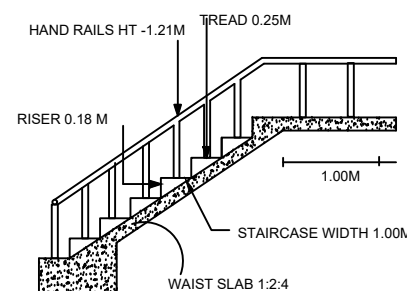
STAIRCASE DETAILS
