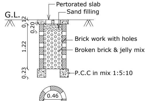
PERCOLATION PIT FOR 30 Sq. m. (Scale:- 1:50)
