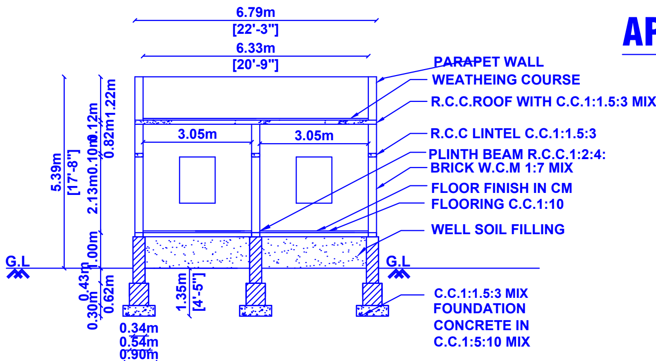
SECTION ON G1G2"
