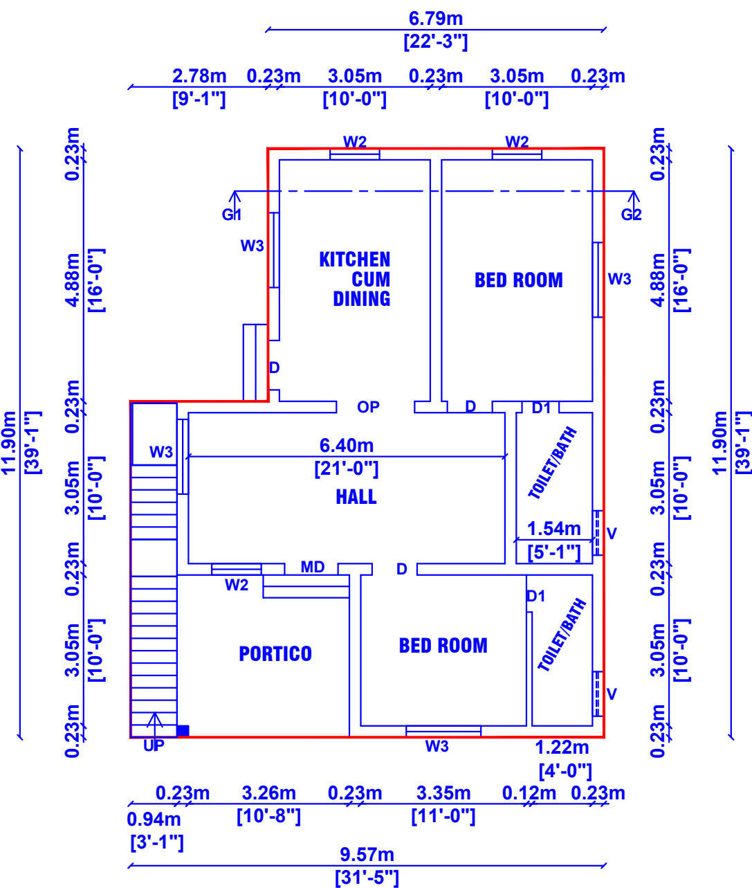
PLAN (Proposed)
