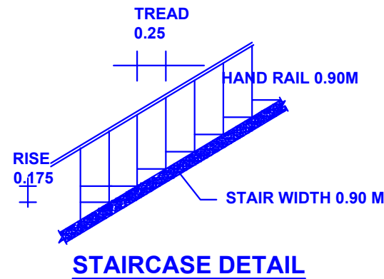
STAIRCASE DETAIL
