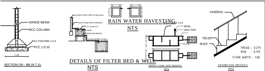
STAIRCASE DETAILS
