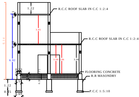
SECTION AB
