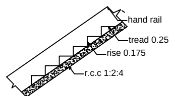
STAIR
