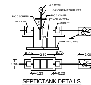
SEPTICTANK DETAILS
