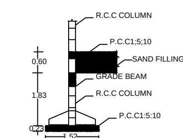
COLUMN DETAILS
