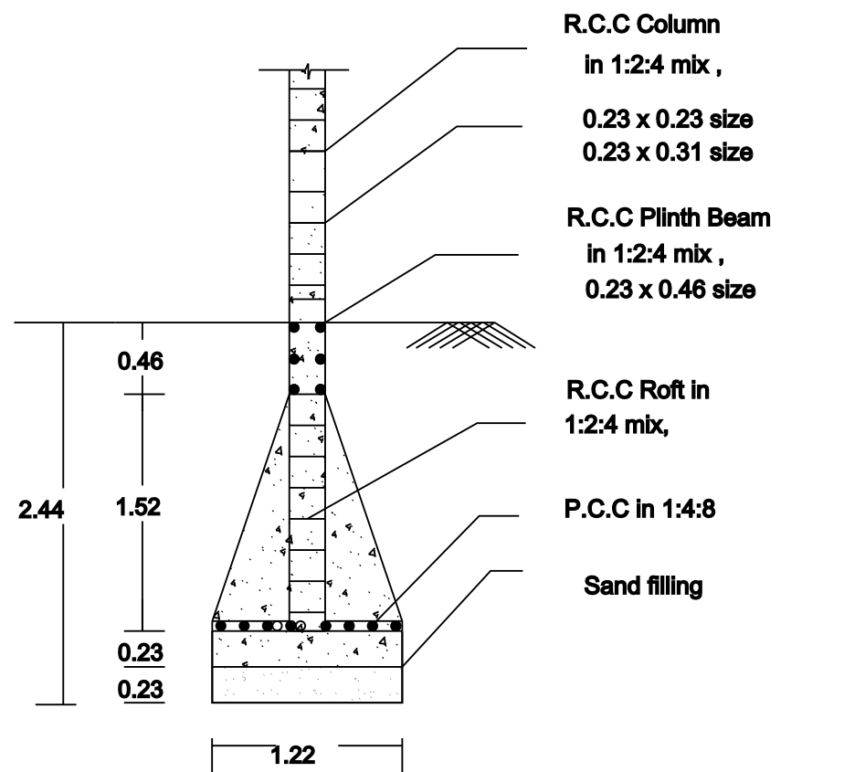
COLUMN DETAILS
