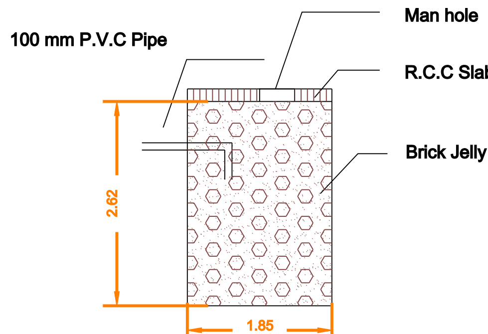
RAINWATER COLLECTION TANK
