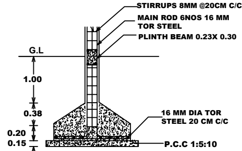
DETAILS OF COLUMN FOOTING
