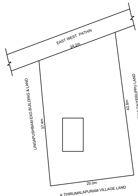
SITE PLAN
