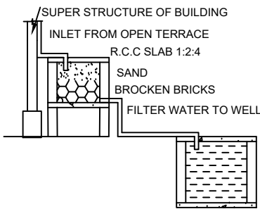
RAINWATER HARVESTING
