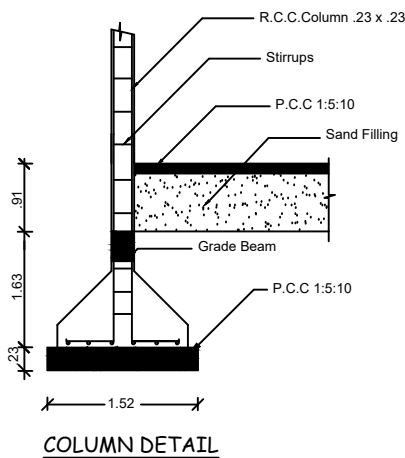
COLUMN DETAIL
