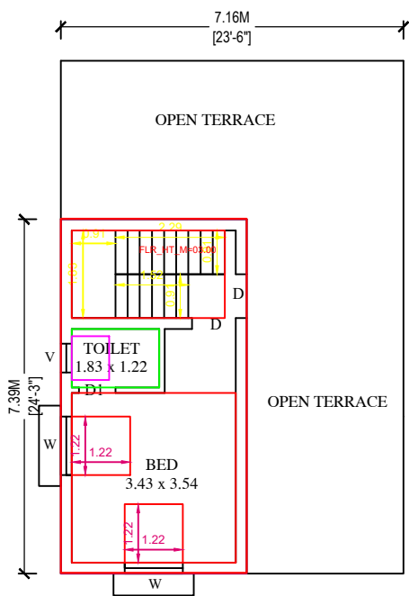
PRO.FIRST FLOOR PLAN
