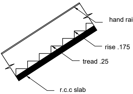
STAIR
