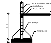
Column Detail
