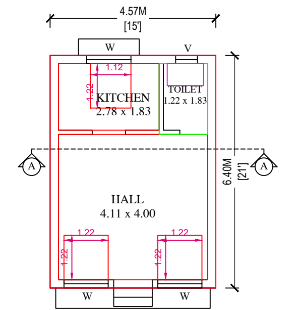
PRO.GOUND FLOOR PLAN
